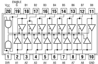
74245 Octal Bus Transceivers 3-State
