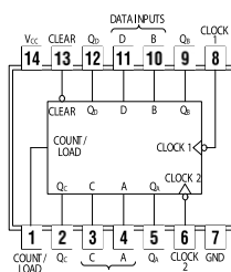
74196, 74197 Presettable Decade Counter Presettable Binary Counter
