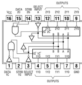
74155, 74156 Dual 2-to-4 Line Decoders/Demultiplexers
