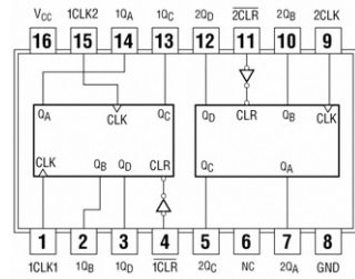
7468, 7469 Dual 4-Bit Decade Counters Dual 4-Bit Binary Counters
