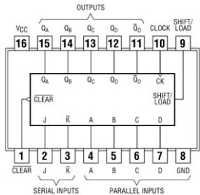
74195 4-Bit Parallel Access Shift Registers
