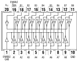
74622 Octal Bus Transceiver O.C.
