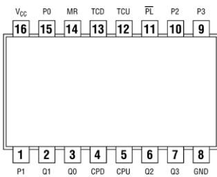
74192 Presettable Synchronous 4-Bit Up/Down Counters
