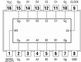
74399 Quad 2-Input Multiplexer with Storage
