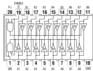
74643, 74644 Octal 3-State Bus Transceivers
