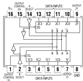
74353 Dual 4-to-1 Line Data Selector 3-State
