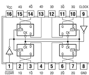
74175 Quad D-Type Flip Flops
