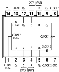
74176, 74177 Presettable Decade Counter Presettable Binary Counter
