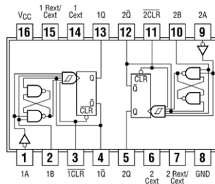
74221 Dual Monostable Multivibrators
