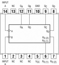
7492 Divide-by-12 Counters
