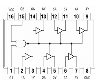
74365 Hex Bus Drivers Hex Buffers/Line Drivers 3-State
