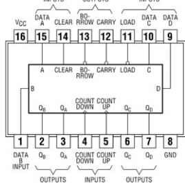
74196, 74197 Presettable Decade Counter Presettable Binary Counter
