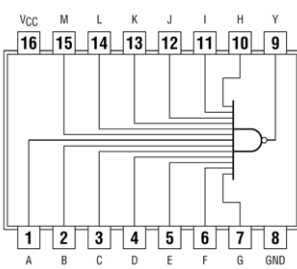
74133 13-Input NAND
