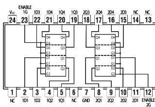
74100 8-Bit Latches
