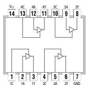
74426 Quad 3-State Buffers
