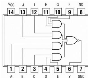
7454(74LS54) 4 wide 2-Input AND-OR-INVERT
