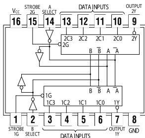
74352 Dual 4-to-1 Line Data Selector
