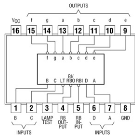
74246, 74247 BCD-to-Seven Segment Decoders
