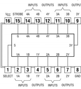
74157, 74158 Quad 2-to-1 Line Data Selectors/Multiplexers
