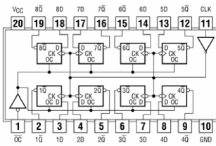
74534 Octal D-Type Edge-triggered Flip Flops
