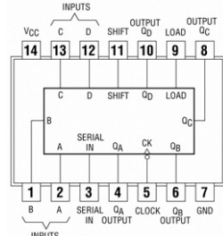
74178 4-Bit Register PIPO
