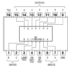
74248, 74249 BCD-to-Seven Segment Decoders
