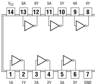
7419 Hex Schmitt Trigger Inverters
