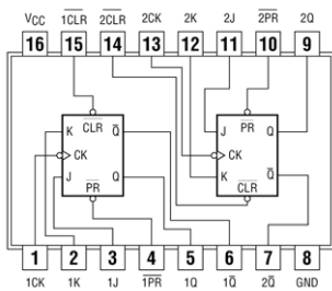
74112 Dual J-K Flip Flops with Preset and Clear
