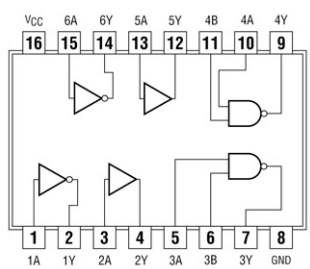
7431 Delay Elements
