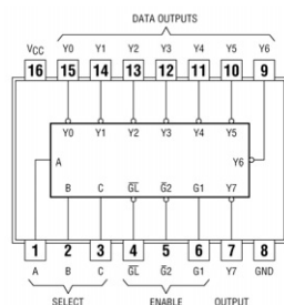
74137 3-to-8 Line Decoders/Demultiplexers Latch
