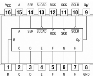
74597 8-Bit Shift Registers
