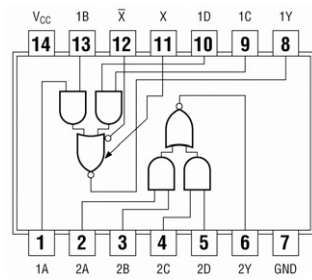
7453 4 wide 2-Input AND-OR-INVERT
