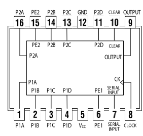
7494 4-Bit Shift Register
