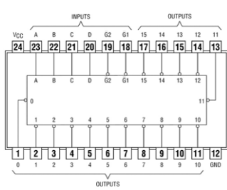
74154 4-to-16 Line Decoders/Demultiplexer
