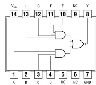
7455 Expandable 2 wide 4-Input AND-OR-INVERT
