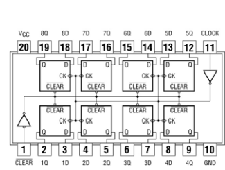
74273 Octal D-Type Flip Flops
