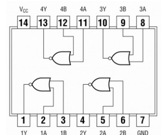
7433 Quad 2-Input NOR Buffers O.C.
