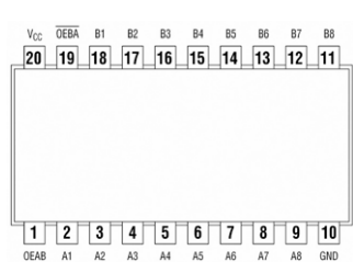
74620, 74621, 74623 Octal Bus Transceivers 3-State
