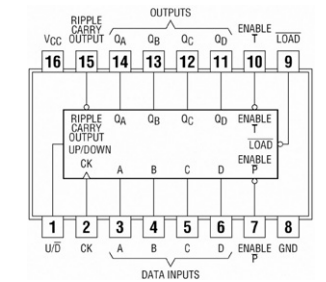
74668, 74669 Presettable Synchronous 4-Bit Up/Down Binary Counter
