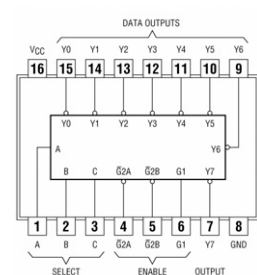
74138 3-to-8 Line Decoders/Demultiplexers
