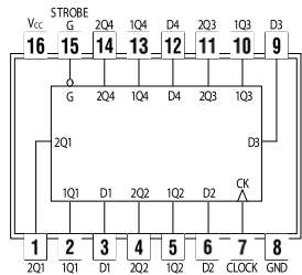
74396 Octal Storage Register
