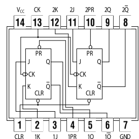
74114 Dual J-K Flip Flops with Preset and Clear
