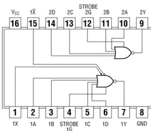
7423 Expandable Dual 4-Input NOR with strobe
