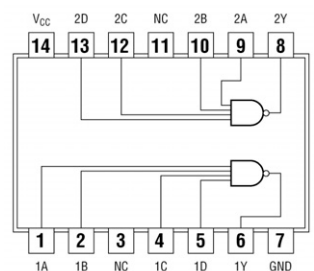
7440 Dual 4-Input NAND Buffers
