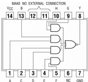
7454 4 wide 2-Input AND-OR-INVERT
