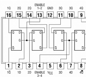
7475 4-Bit Bistable Latches
