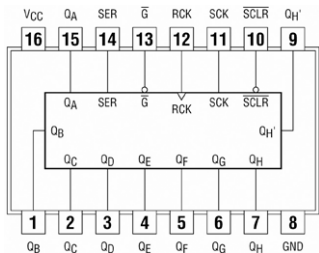
74595, 74596 8-Bit Shift Registers
