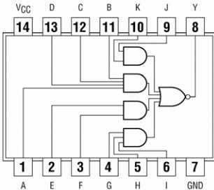
7464 4-2-3-2 Input AND-OR-INVERT
