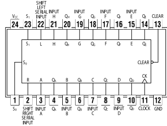
74198 8-Bit Bidirectional Shift Register PIPO
