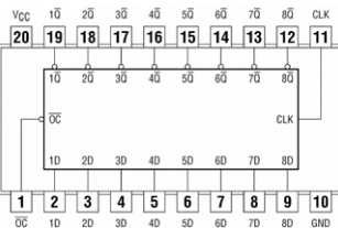
74564 Octal D-Type Flip Flops
