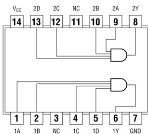
7421 Dual 4-Input AND
