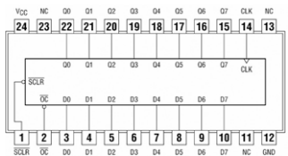
74575 Octal D-Type Edge-triggered Flip Flops
