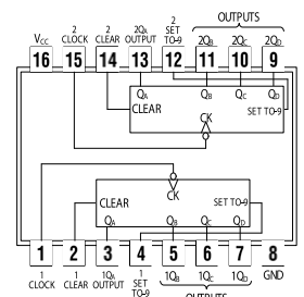
74490 Dual Decade Counters
