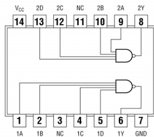
7422 Dual 4-Input NAND O.C.
