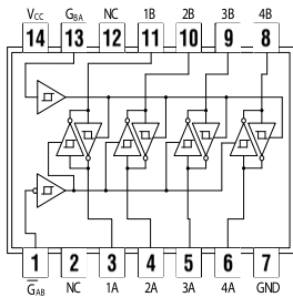
74242 Quad Bus Transceiver
