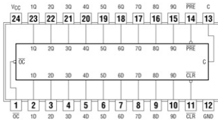
74843 9-Bit Bus Interface D-type Latches with 3-state Outputs
