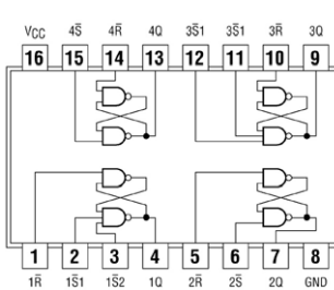
74279 Quad S-R Latches
