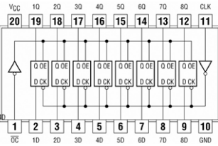
74574 Octal D-Type Edge-triggered Flip Flops
