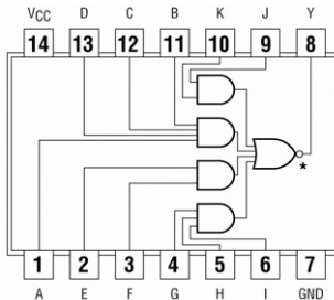
7465 4-2-3-2 Input AND-OR-INVERT O.C.
