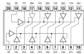
74244 Octal Bus Drivers 3-State
