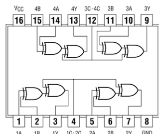
74135 Quad 2-Input XOR/XNOR
