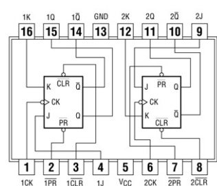
7476 Dual J-K Flip Flops with Preset and Clear
