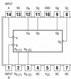
7493 4-Bit Binary Counters
