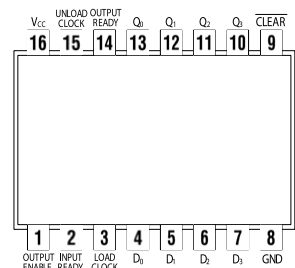
74224 16x4 Synchronous FIFO Memory with 3-State Outputs
