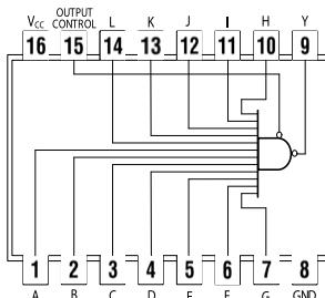
74134 12-Input 3 States NAND
